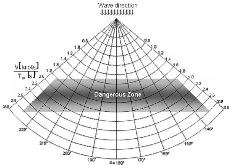
Figure 3: Risk of successive high wave attack in following and quatering seas
