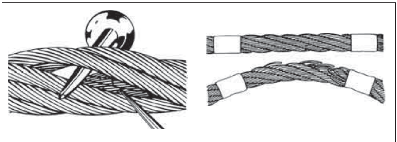
Fig.4 Inspections of rope for internal and external damage (by courtesy of Certex (UK))
