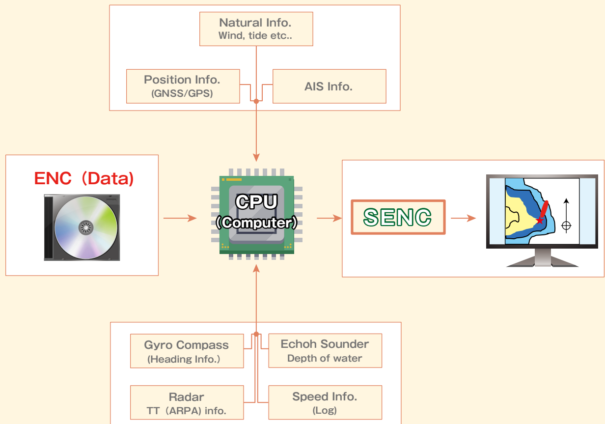
Figure : 7 Structure of ECDIS
