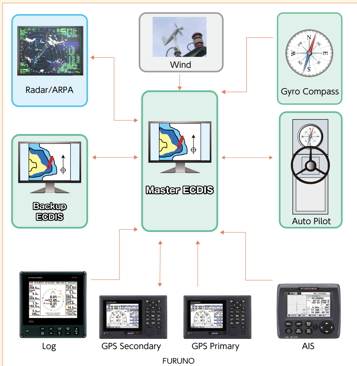
Figure : 15 ECDIS and other Nautical Equipment
